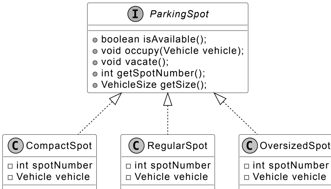
Parking Spot and its concrete classes
