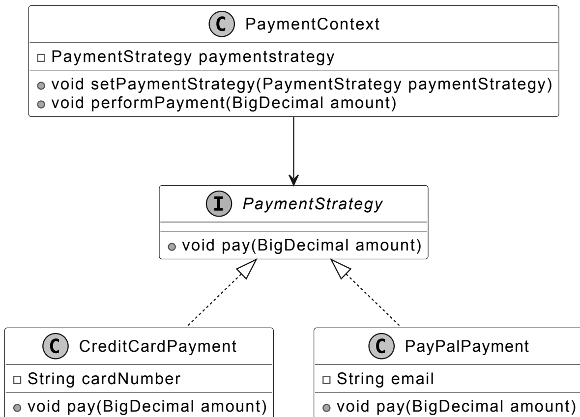
Strategy design pattern class diagram
